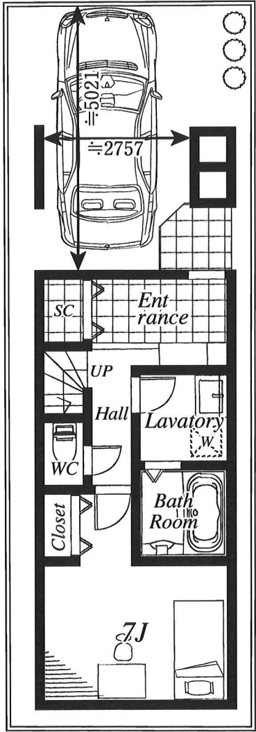
1F 29.81㎡
