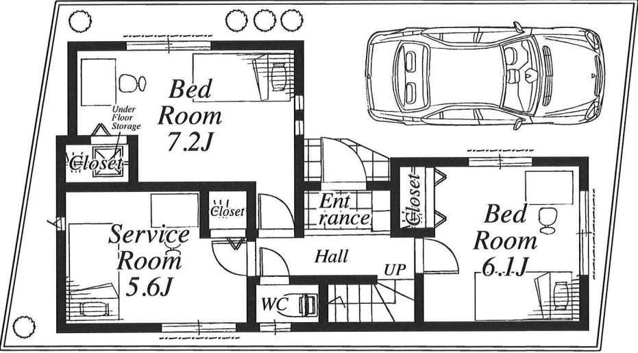
1F 40.99㎡
